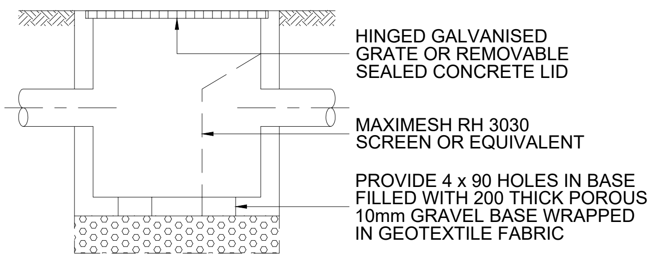
SILT ARRESTOR PIT WITH SCREEN
